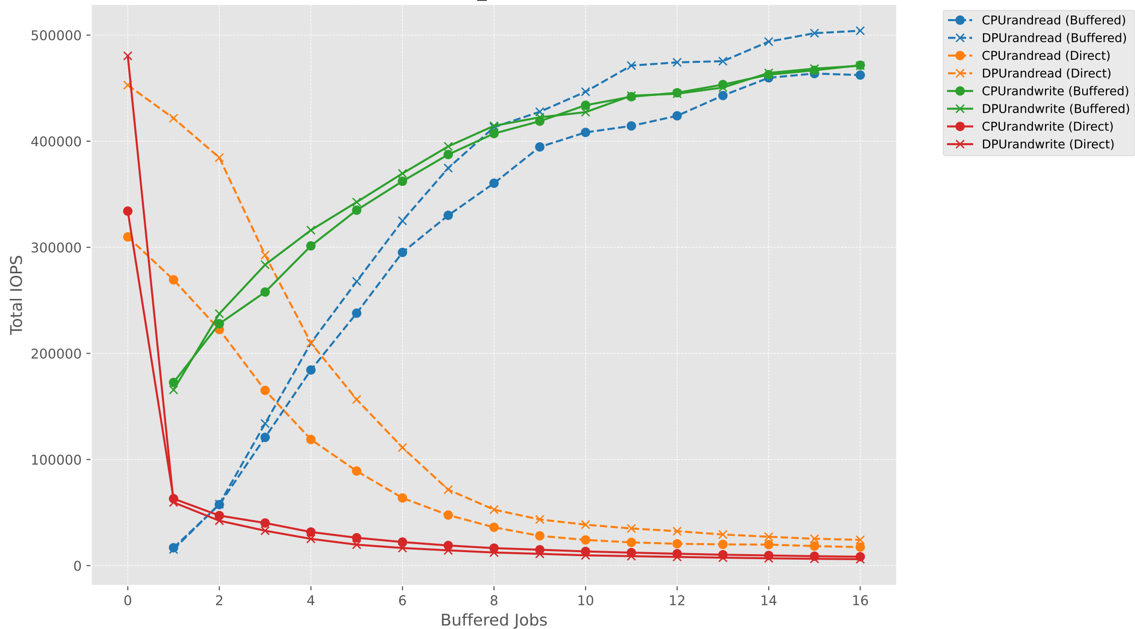
IOPS vs Buffered Jobs (direct1_bufferedN) - RAND (CPU vs DPU)
